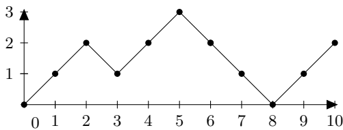
A sample generalized Dyck path of type (10, 2)
