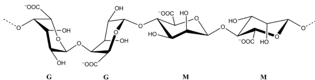
Fig. 1. Structure of alginates [4].
