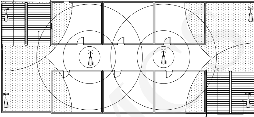
Fig. 6. Limiting WLAN range by set a of antennas
