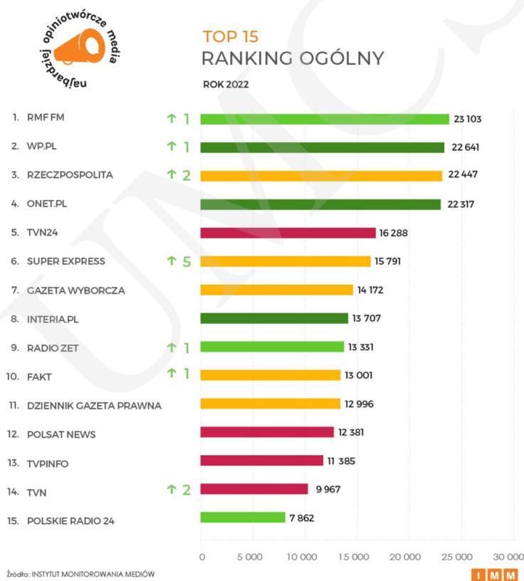
Figure 2. Results of press citations research – general ranking
